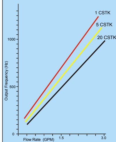
Figure 6 VISCOSITY EFFECTS ON MF175
