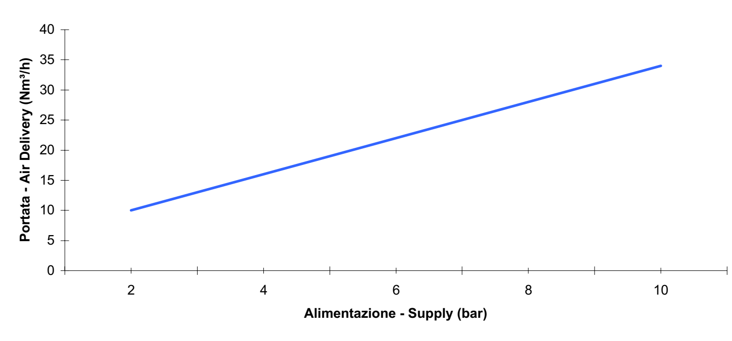
DIAGRAMMA PORTATA - AIR DELIVERY DIAGRAM
