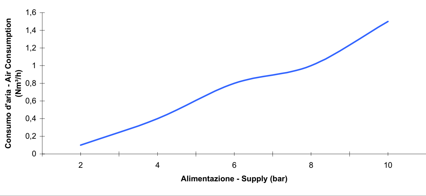
DIAGRAMMA CONSUMI - AIR CONSUMPTION DIAGRAM
